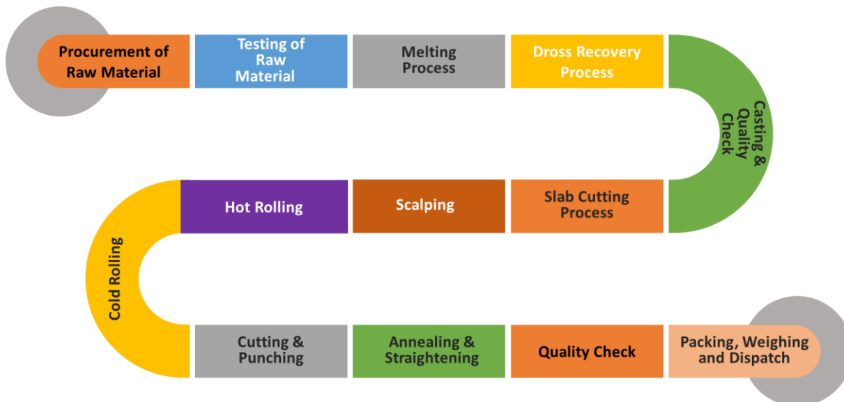
Flow Chart of Manufacturing of Aluminium Circles, Sheets and Slabs
